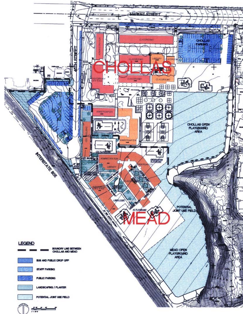
MEAD ELEMENTARY SCHOOL CONCEPTUAL DESIGN
